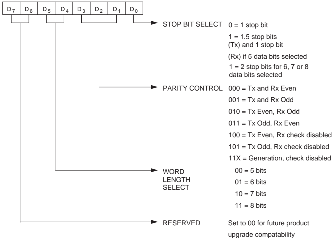
Figure 2-8: UCR
