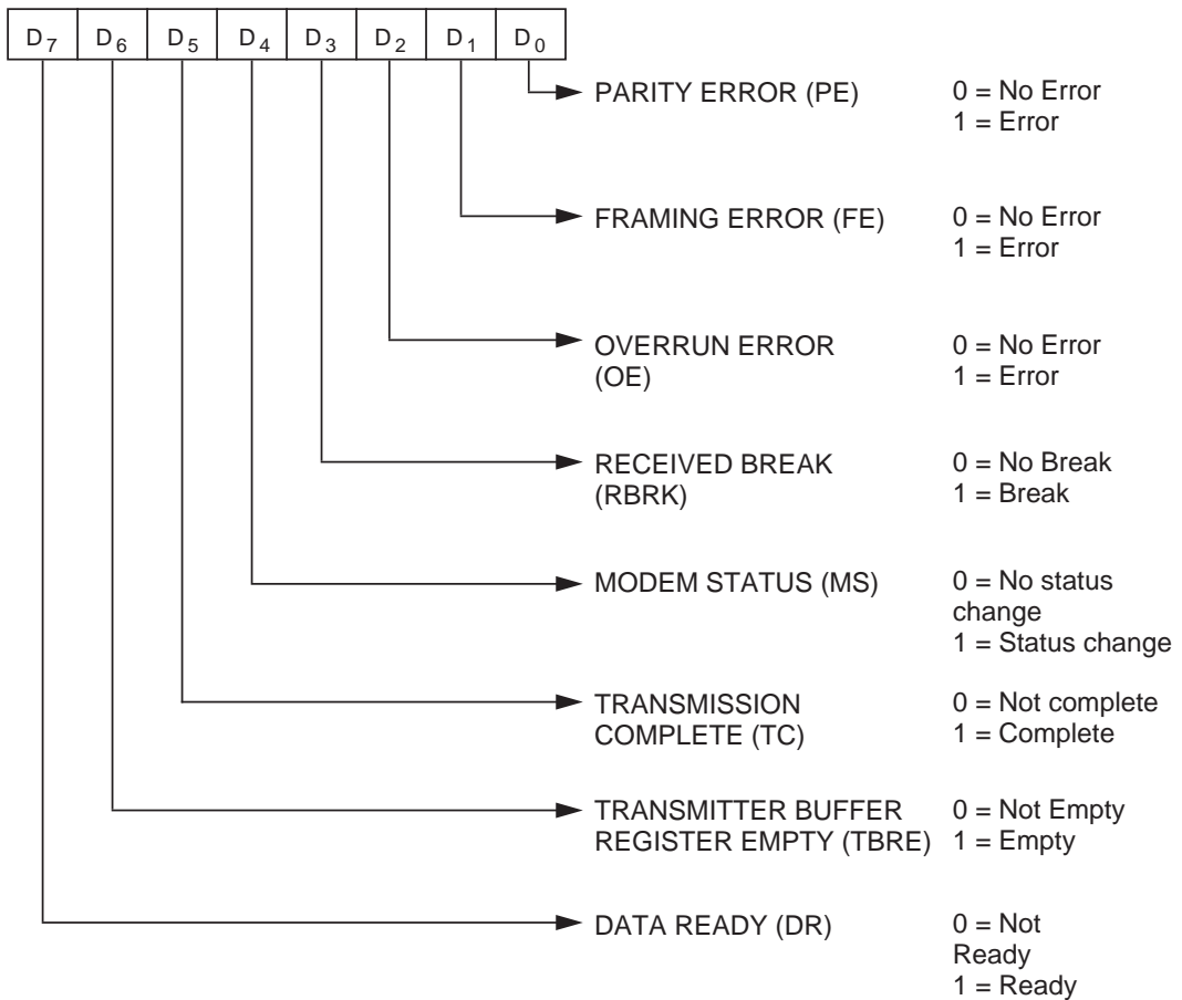
Figure 2-12: USR
