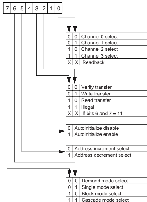
Figure 2-12: Mode Register
