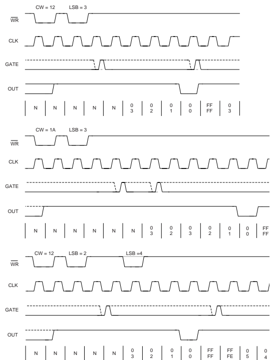
Figure 2-17: Mode 5 Timing
